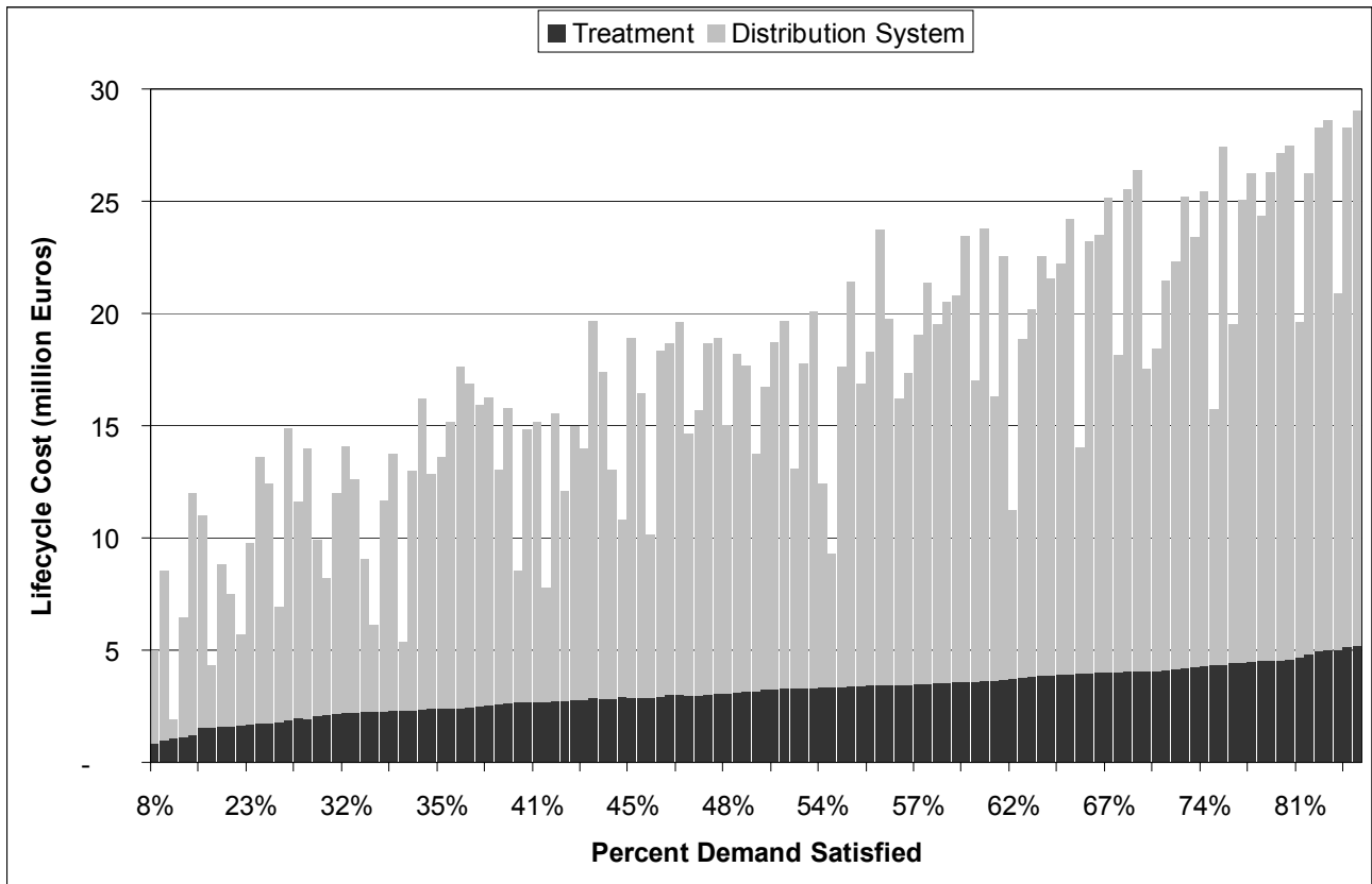
Figure 4 Life cycle cost of different reuse scheme options
