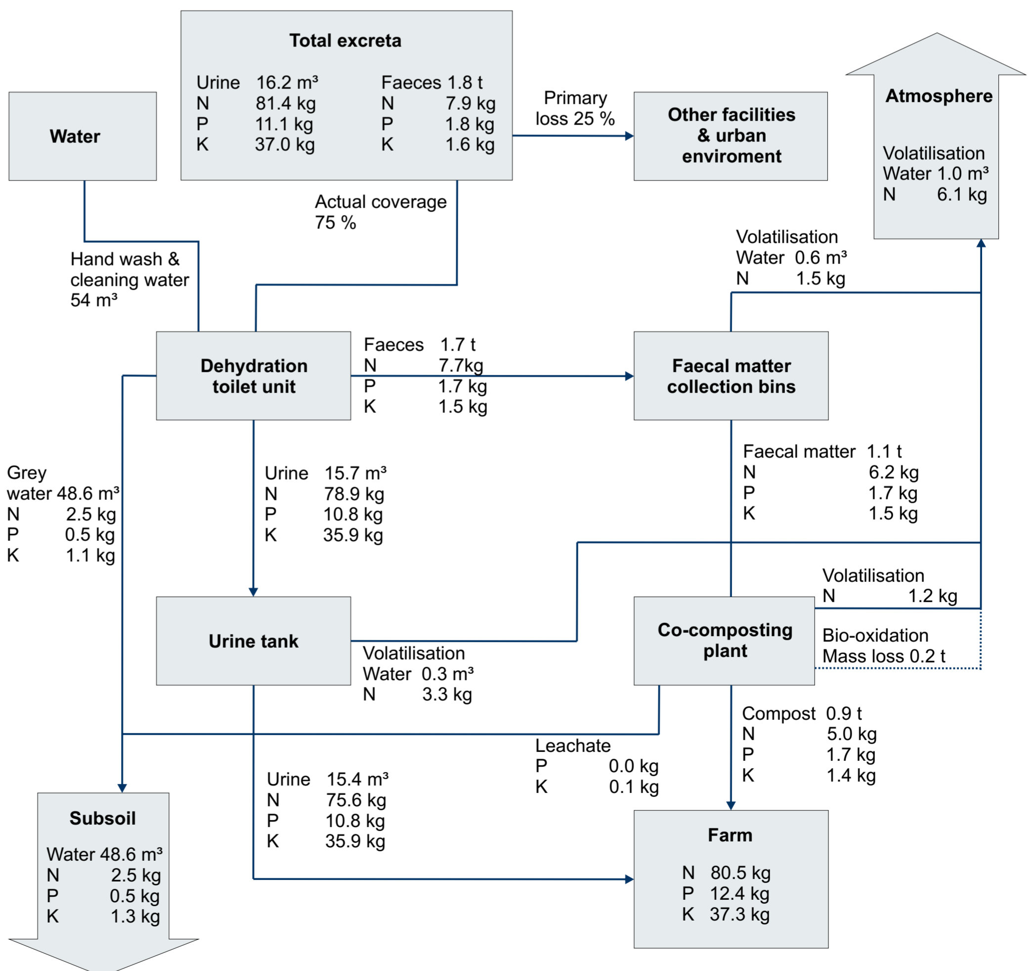
Estimated monthly mass and nutrient flows of a BBT dehydrating toilet unit serving 600 people
