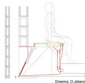
Side view of the toilet box and the shaft
